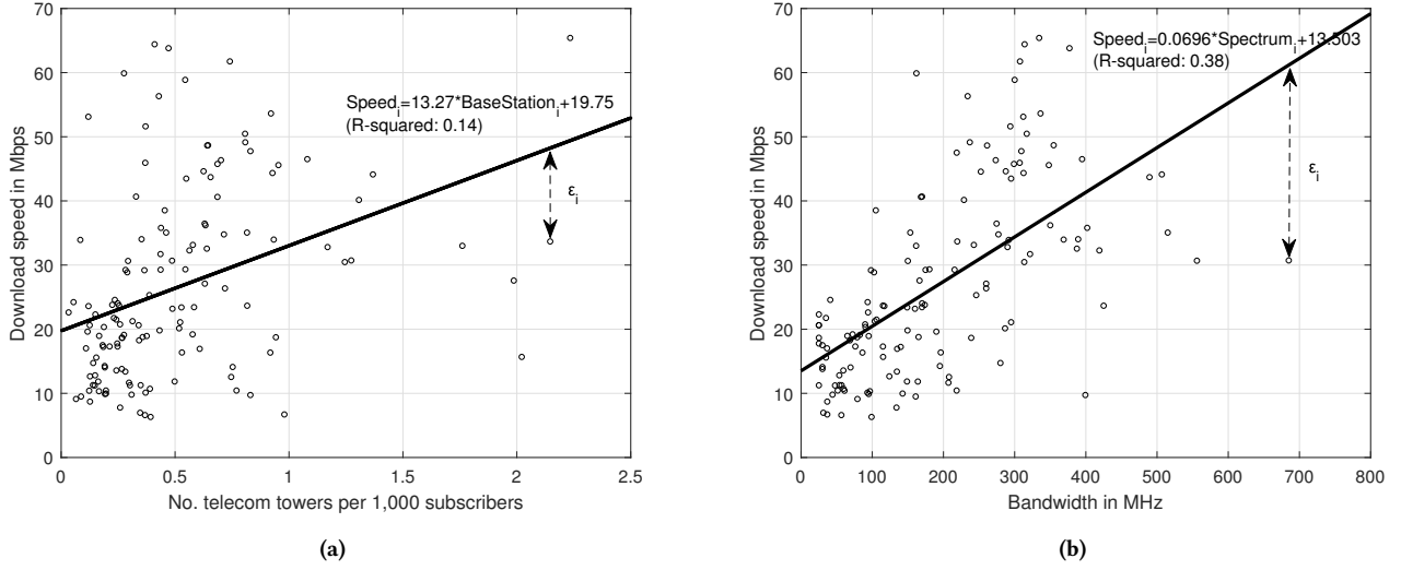
Figure 2: Two simple linear regression examples: (a) the number of telecommunication towers; (b) bandwidth.
